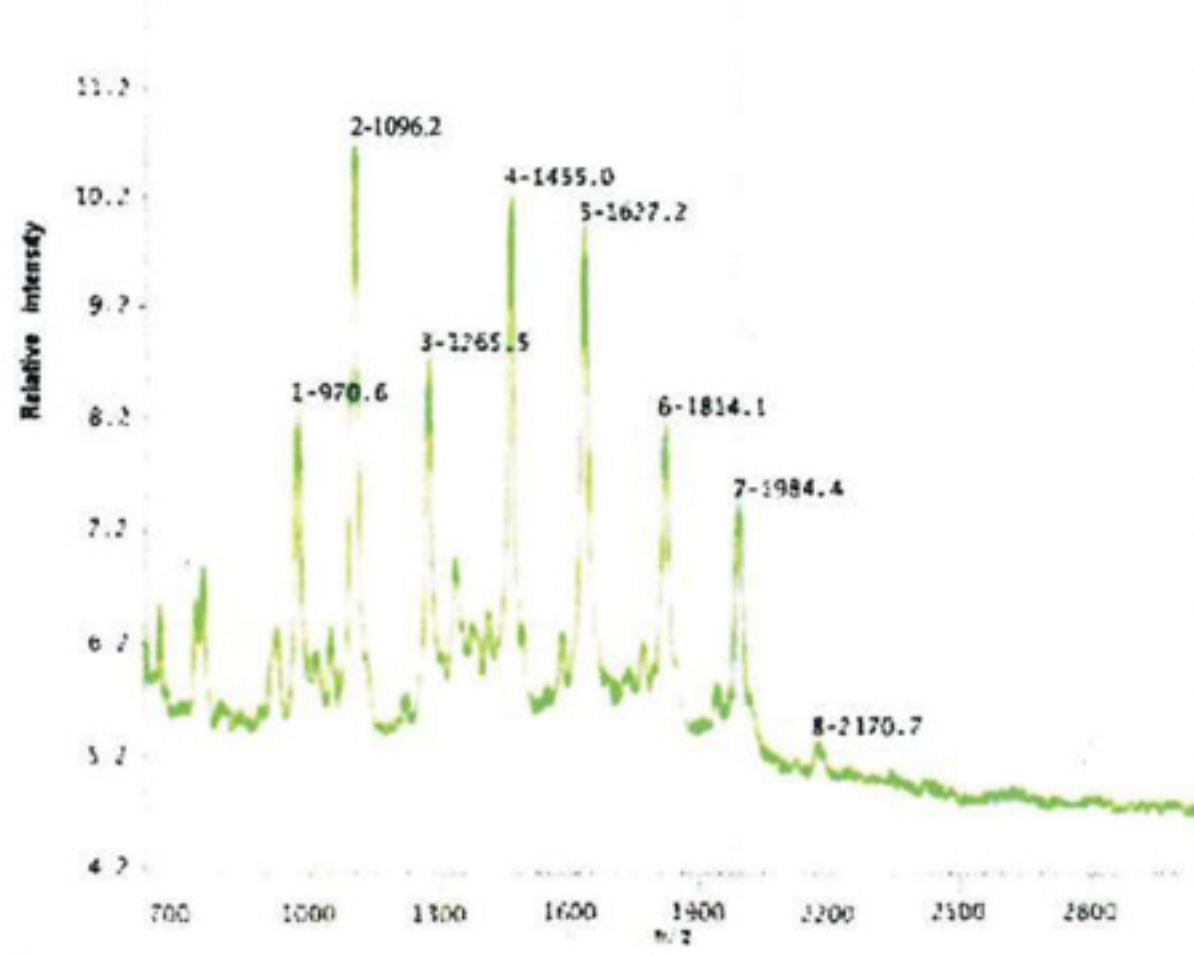
Fig. 2: UV-Maldi-ToF mass spectrum of SiS AM 500 (3-trimethoxyl-quat [1096-2]) After 2000 hours accelerated weathering.
